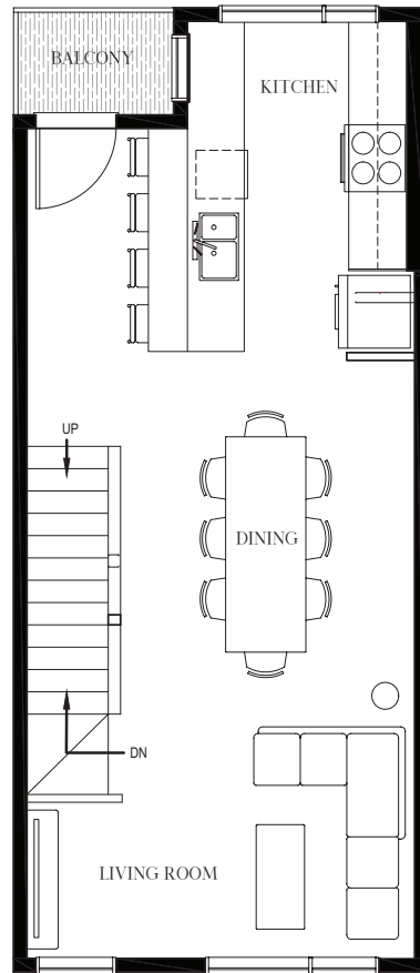
SECOND FLOOR 484 SQ. FT.
