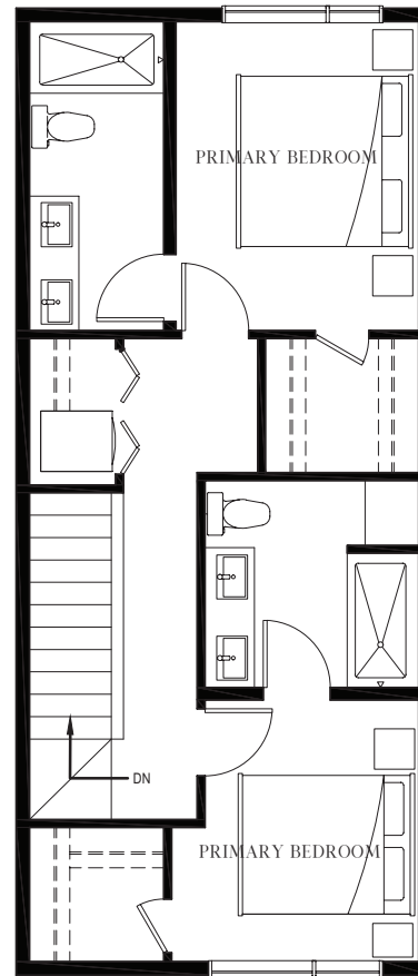
THIRD FLOOR 508 SQ. FT.
